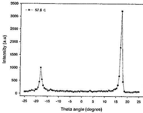
Fig. 4. The theta scan of pure Felix-015/100 at 57.6 °C. The peak positions are symmetric but the intensity of the peaks is not symmetric.
