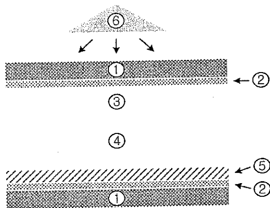
Fig. 1. Schematic of the structure of a PSCOF cell. ① glass substrates, ② electrodes, ③ polymer region, ④ LC region, ⑤ alignment layer, and ⑥ UV source.
