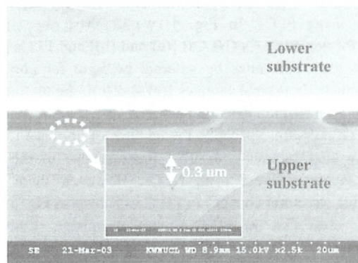
Fig. 3 Cross section image of PILC sample using scanning electron microscope. The inset is the magnification of dotted circle.
