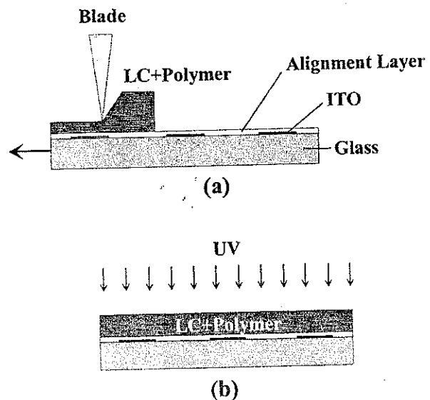
Figure 1. Schematic illustration of the fabrication process.
