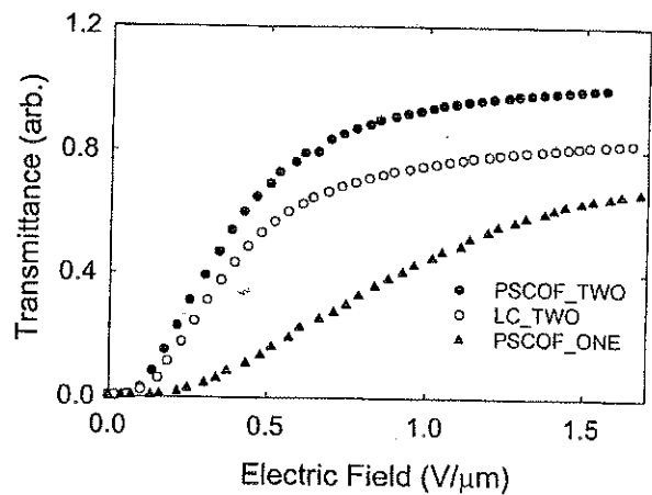
Figure 6. Transmission vs. Applied field for the one substrate (PSCOF_ONE), two-substrate (PSCOF_TWO), and normal IPS cell (LC_TWO).
