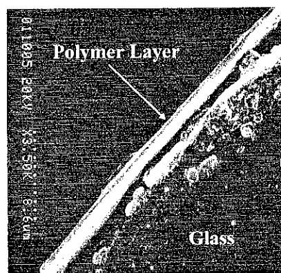
Figure 3. SEM image showing substrate and polymer film.
