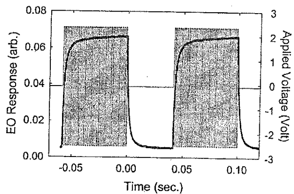
Figure 7. Optical switching behavior
