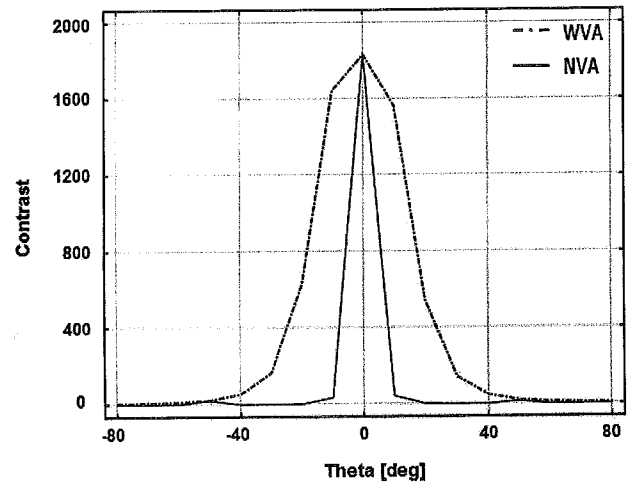
Fig. 6. The contrast ratios of the WVA ( \Delta nd = 0.0 ) and NVA ( \Delta nd = 2.2 ) modes along the diagonal axis.
