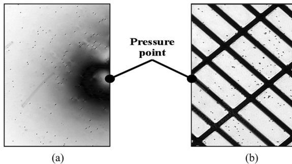
FIGURE 2 Alignment textures of (a) a normal sample and (b) a PILC sample fabricated with the plastic substrates. The polarizing microscopic textures are taken in the presence of an external point pressure with a sharp tip.
