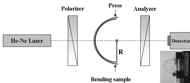
FIGURE 3 Schematic diagram of measurement setup for EO characteristics with respect to bending pressure. The inset is the real image of bending stage with sample.
